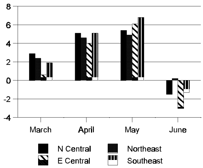
Figure 10. Departures from normal temperatures in four regions in Minnesota during March, April, May and June 1998.
